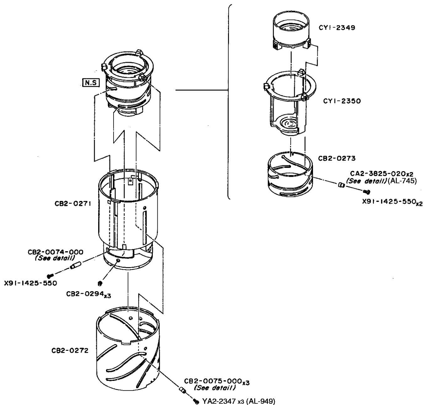
CA2-3825-020 detail
